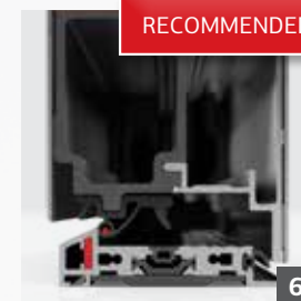
Magnet WeatherSeal sealing
